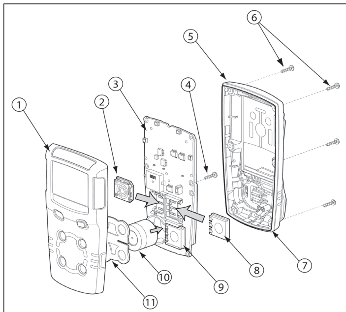
Figure 11. Replacing a Sensor or Sensor Filter
