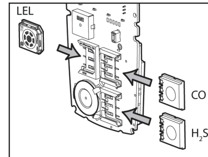
Figure 12. Sensor Positioning
